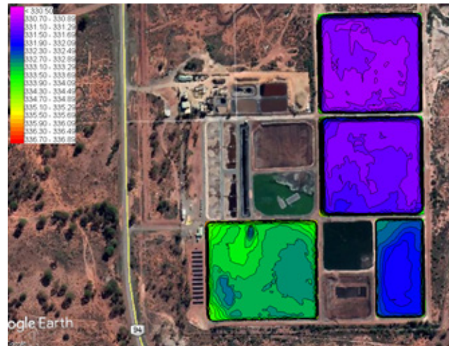
Fig. 8. Sludge Surface Elevation
